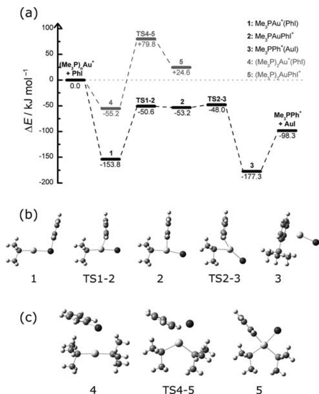
Figure 2. DFT-calculated energy diagrams (at the M06/SDD6-31G-(d,p)/B3LYP/SDD6-31G(d,p) level of theory) for ion-molecule reactions of iodobenzene with a) \text{Me}_3\text{PAu}^+ and (\text{Me}_3\text{P})_2\text{Au}^+ , b) key species for reaction of \text{Me}_3\text{PAu}^+ ; c) key species for reaction of (\text{Me}_3\text{P})_2\text{Au}^+ .
