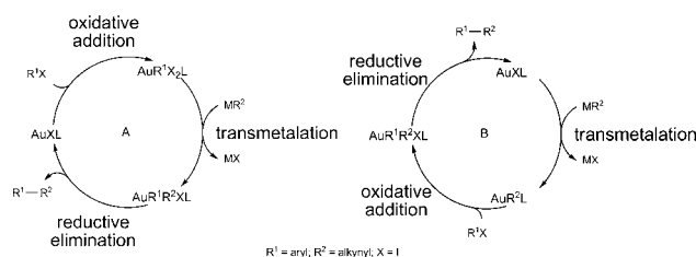
Scheme 2. Catalytic cycles proposed by Lauterbach et al. for an \text{Au}^I complex mediated Sonogashira cross-coupling. [2b] A key requirement for both cycles is oxidative addition. \text{R}^1\text{X} is an aryl halide and \text{MR}^2 is a metal acetylide.
